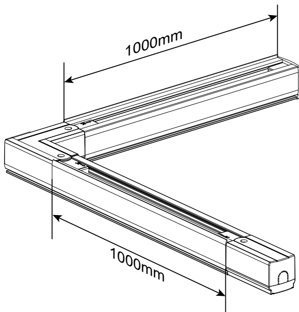
90032/90033 Max. loading 5kg
